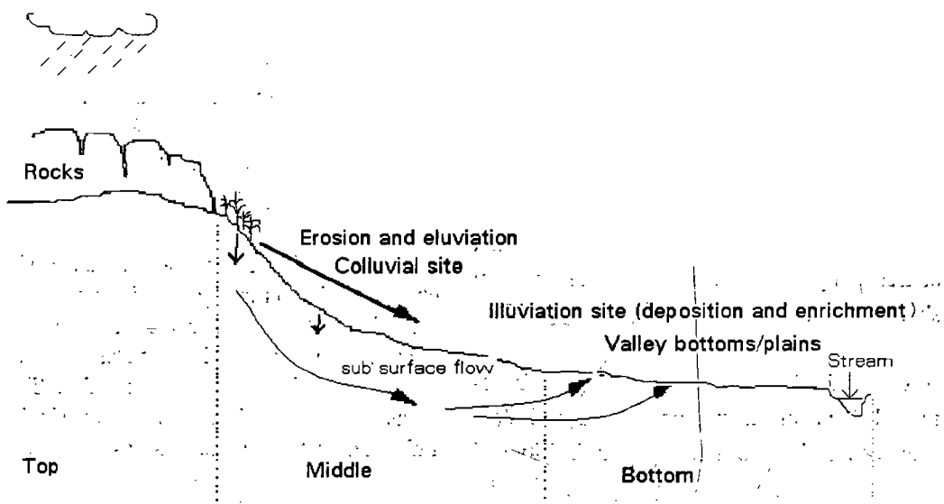
Figure 1: Water movement in a generalised catena
